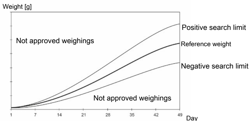
Figure 6: Example of search limit in relation to the reference weight. When the animal type in the controller is set to Males and Females, it is possible to make a positive and a negative adjustment in relation to the search limit.
